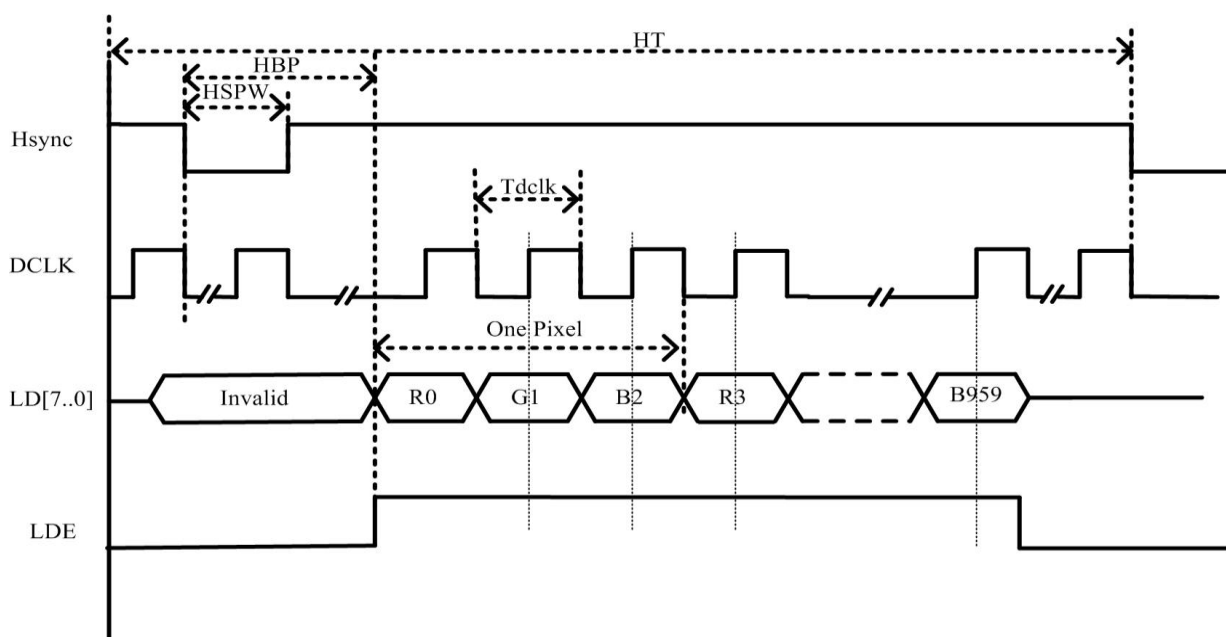
Figure 6-6. Serial Mode Horizontal Timing
