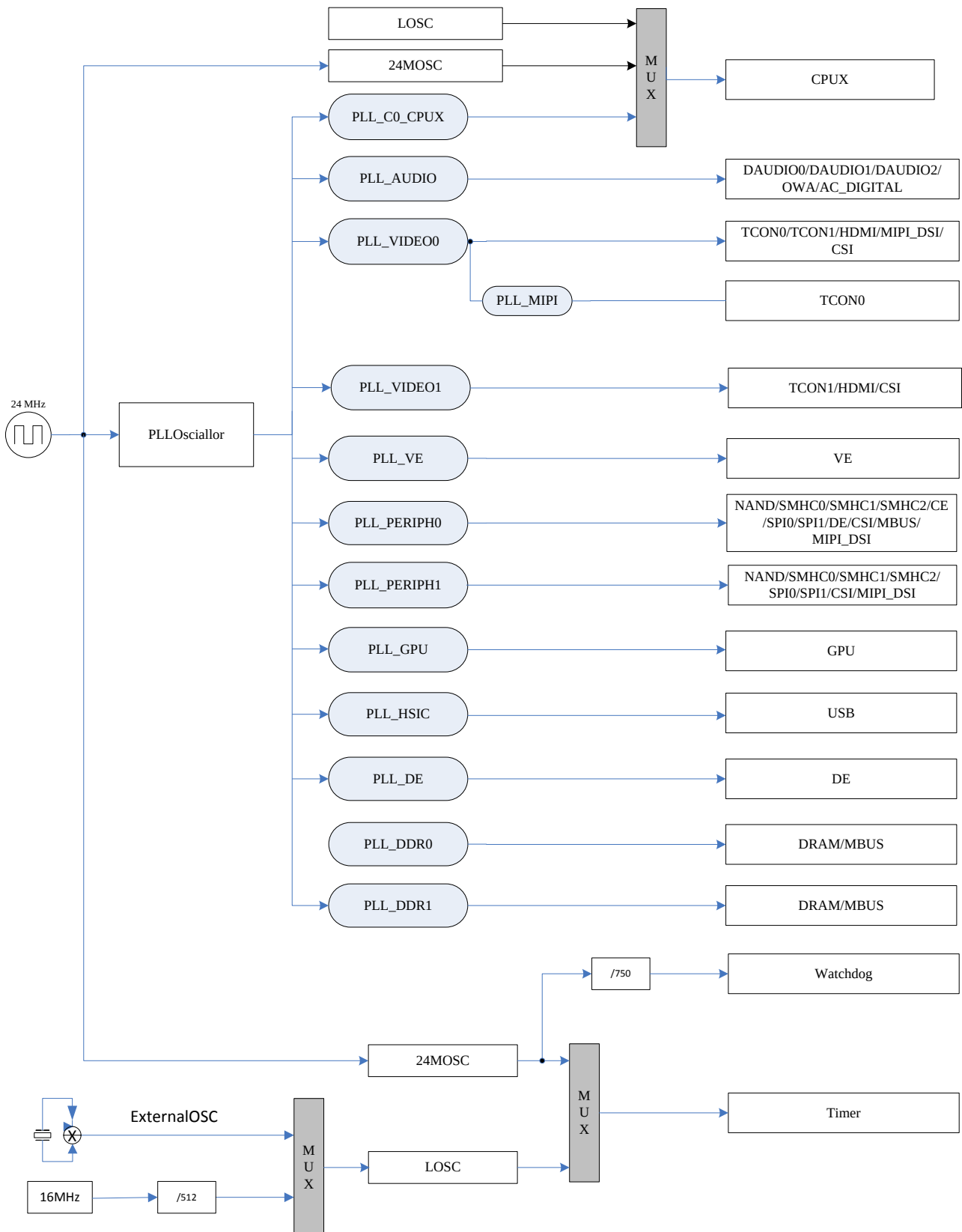
Figure 3-3.Module Clock Diagram
