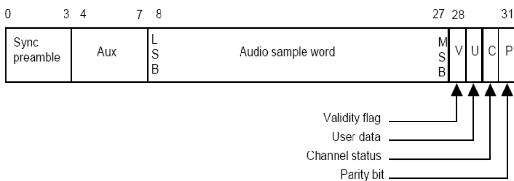
Figure 7-14. Sub-Frame Format
