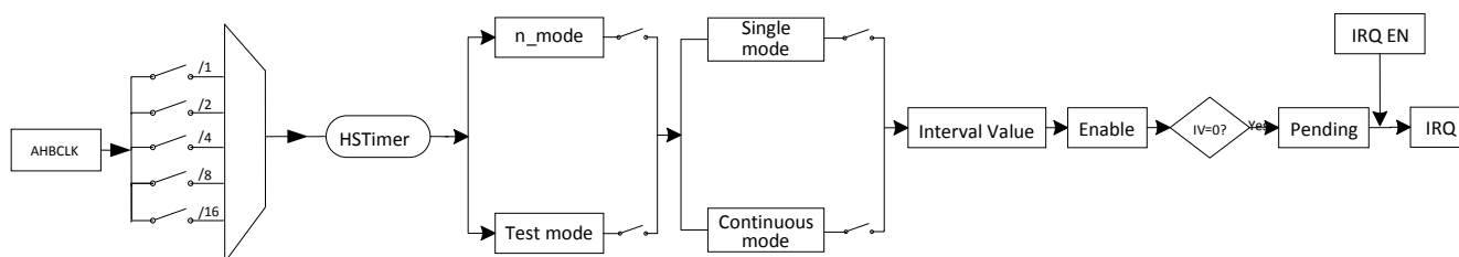
Figure 3-7. HSTimer function structure and work flow
